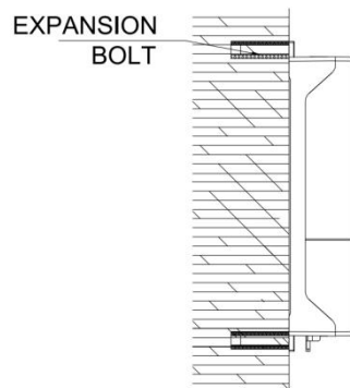
Pic 1 Wall mounted installation
